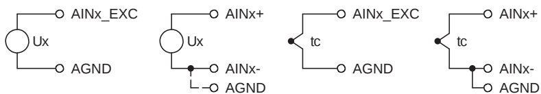
Obr. 1. Wiring diagram for voltage signals and thermocouples.
