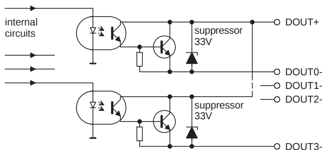
Fig. 4. Simplified diagram of the digital outputs.
