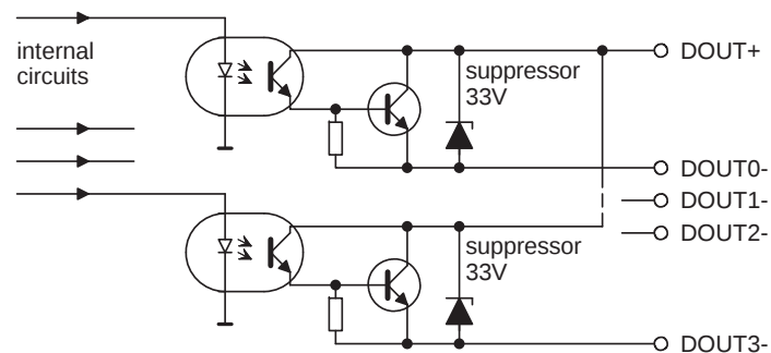
Fig. 3. Simplified diagram of the digital outputs.
